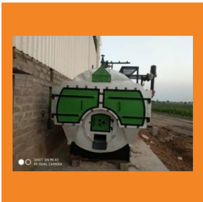
Coal Fired IBR Approved High Pressure Steam Boiler 1000 Kg/hr
